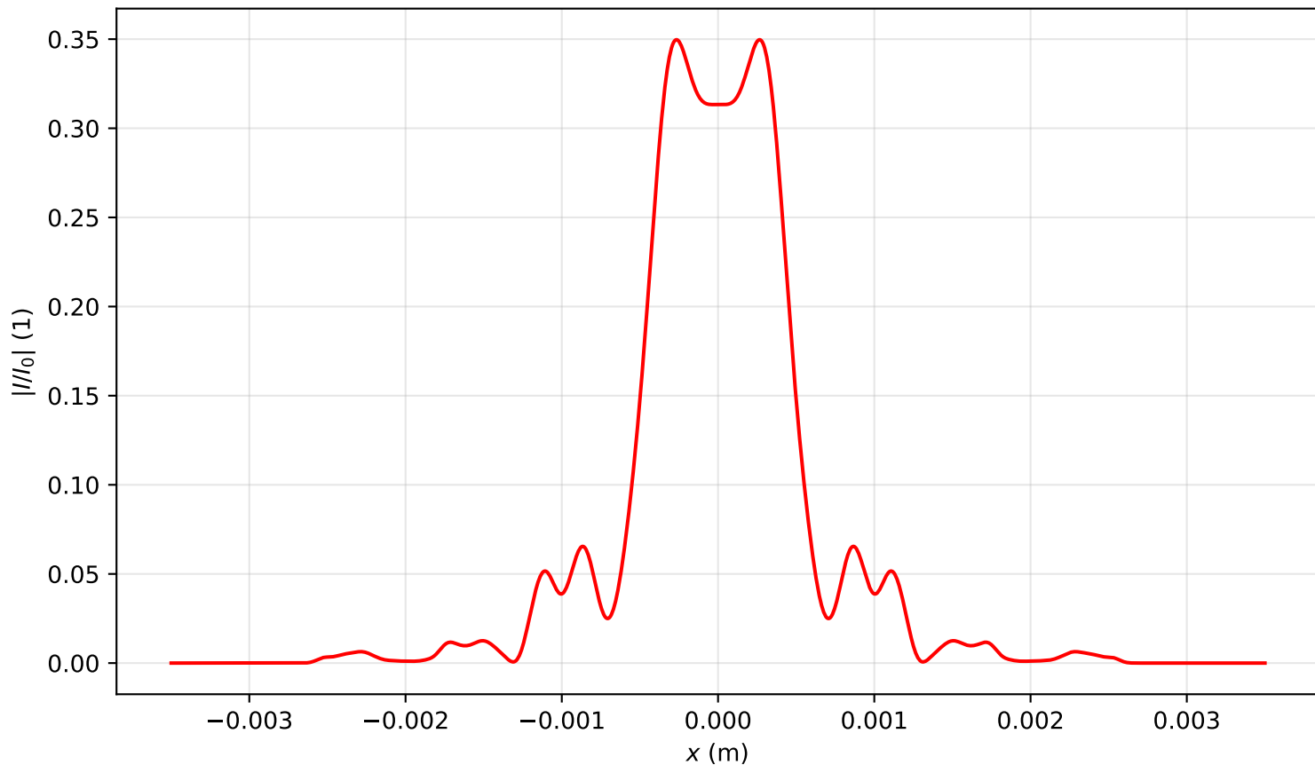
Intensity profile I(x, y = 0, z = 1.911)/I_0 , P_{in}=5.5P_{cr} , artificial time
